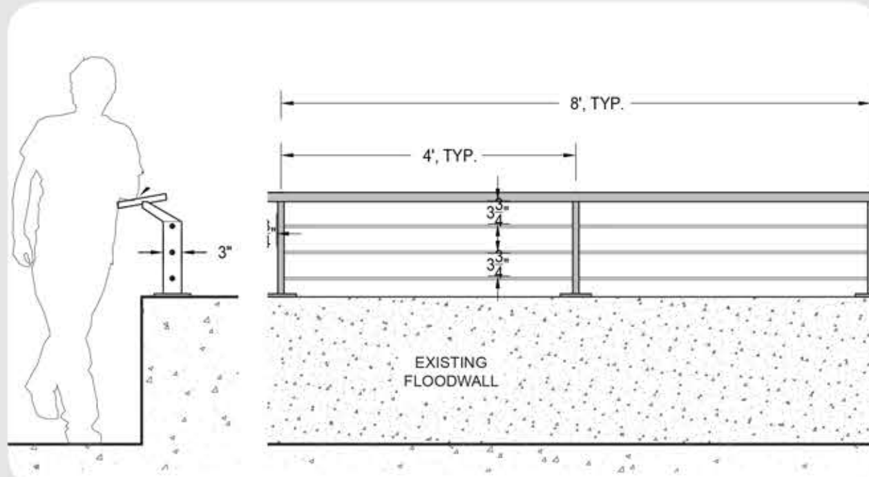
Railing System - On Top of Floodwall
